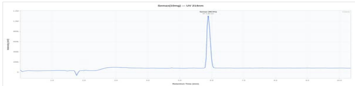
Representative chromatogram, Dedicated V0 (99.53% purity, closest to batch mean of 99.40%)
